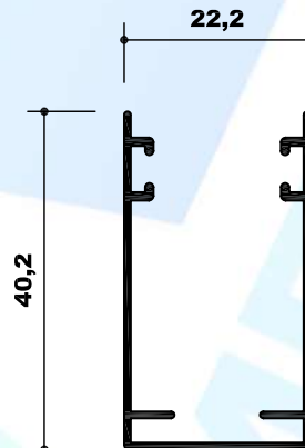
HY2379-37 GUIA MOSQUITERA 40mm
