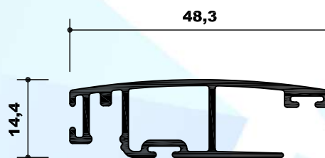
HY2501-37 MOSQUITERA CORREDERA
