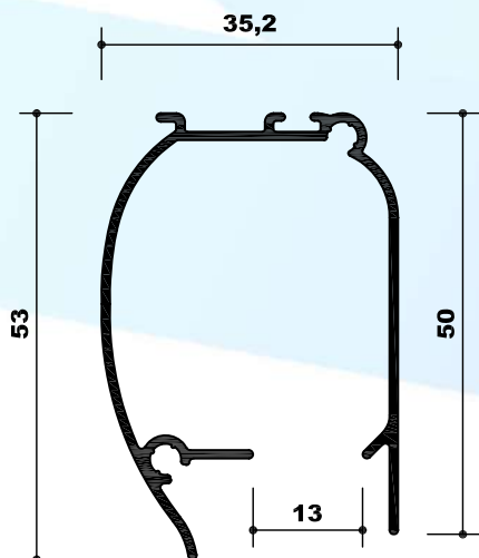
HY2802-37 CABEZAL R35
