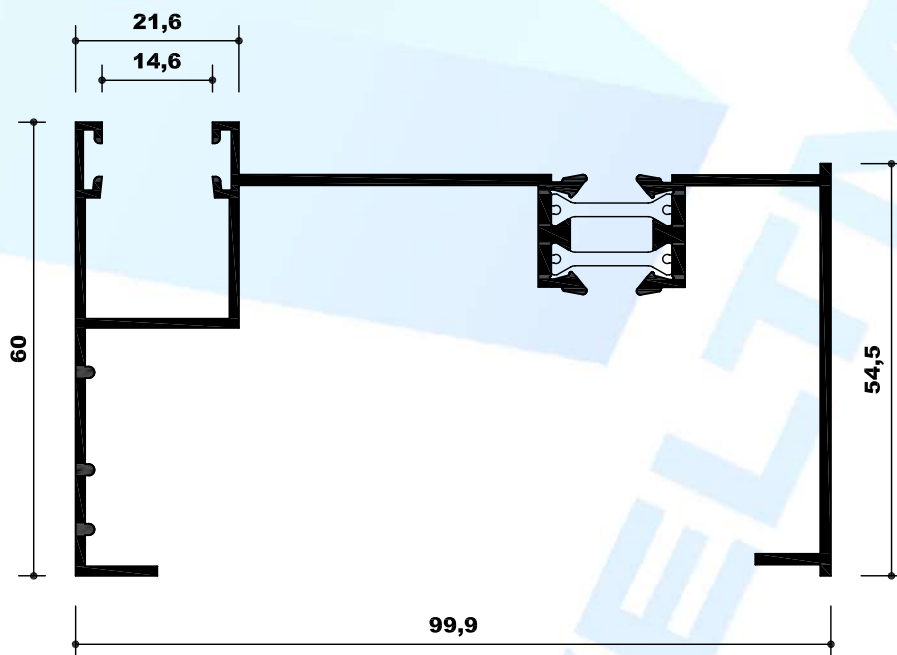
RT-60 GUIA ROTURA 100mm
