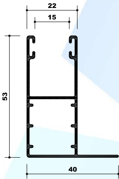
10806 GUIA ALA 53x40 - H25 ALA
