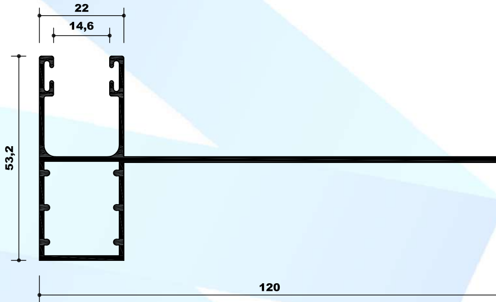
10198 GUIA 120mm DE PALA CENTRAL
