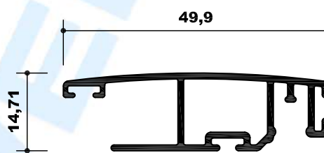
19066 MOSQUITERA CORREDERA PH
