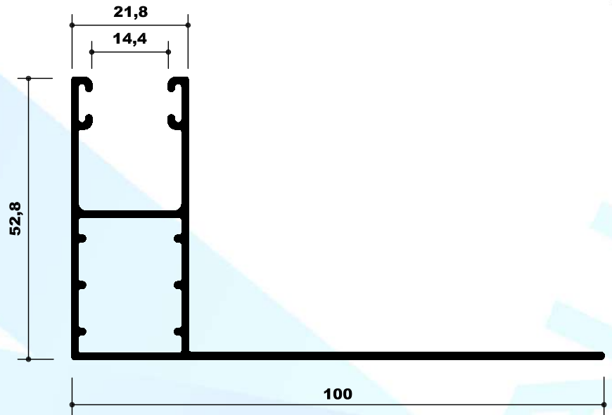
19091 GUIA PALA BAJA 100mm
